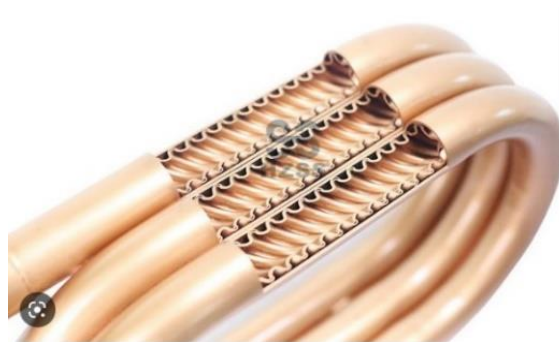
Double Wall Coaxial Coils Heat Exchanger Spirally Corrugated Tubes - Buy Double Wall Coaxial...
